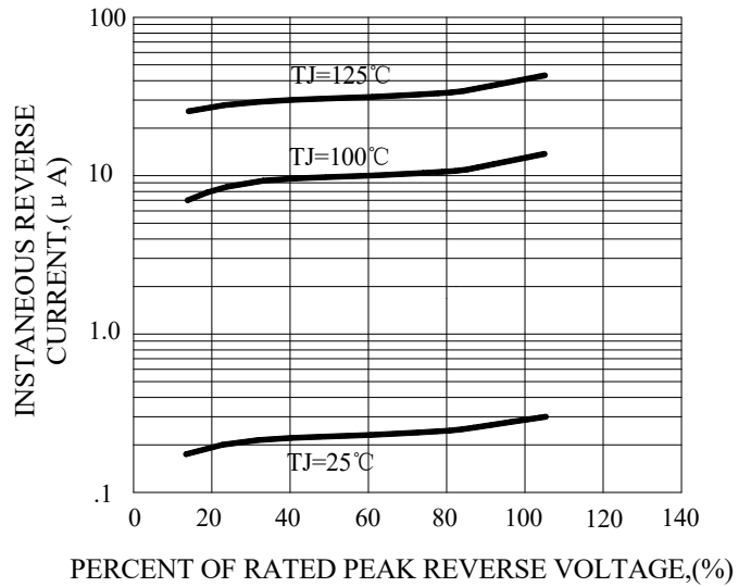
FIG.4-TYPICAL REVERSE CHARACTERISTICS
